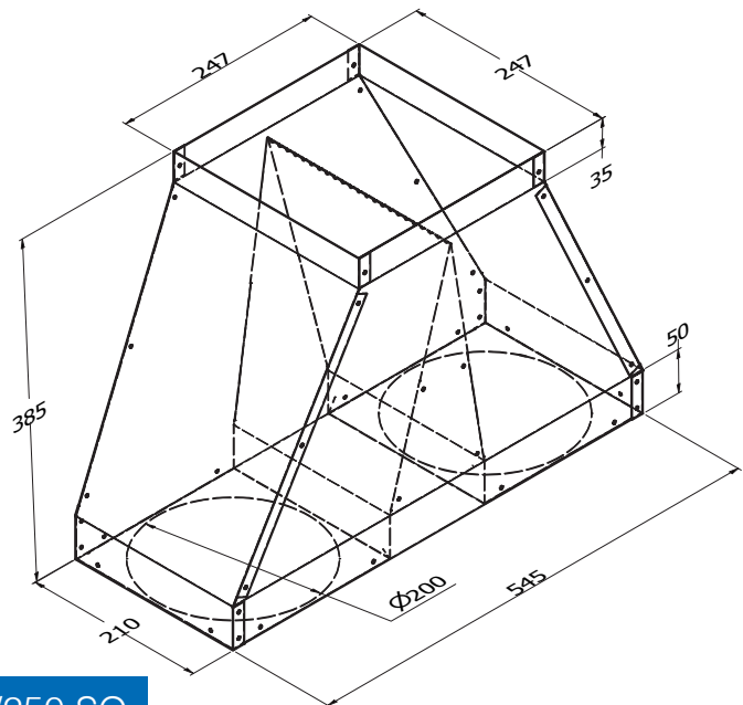
TMT-200/250 SQ
