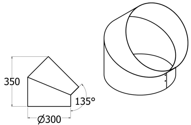
225 DR-300/45°
