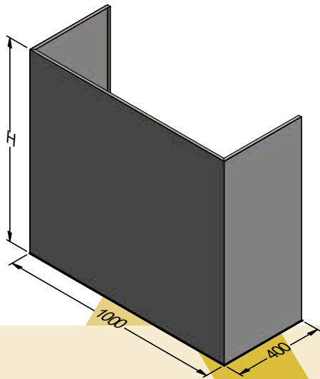
MUR 1000L-2 SHROUD
