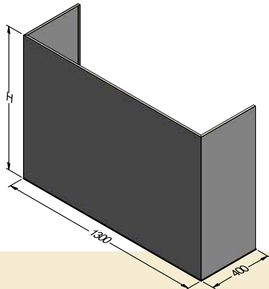
MUR 1300L-3 SHROUD
