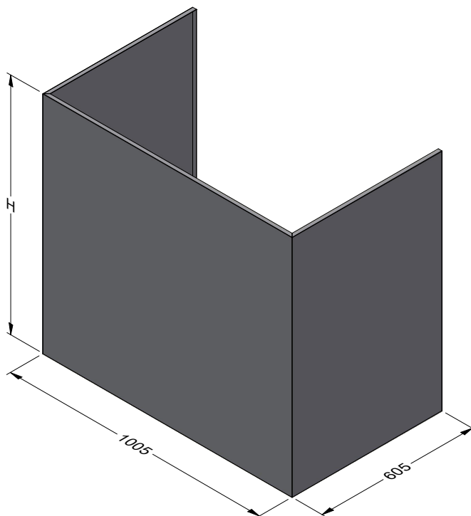
BCM 1200L-3 SHROUD
