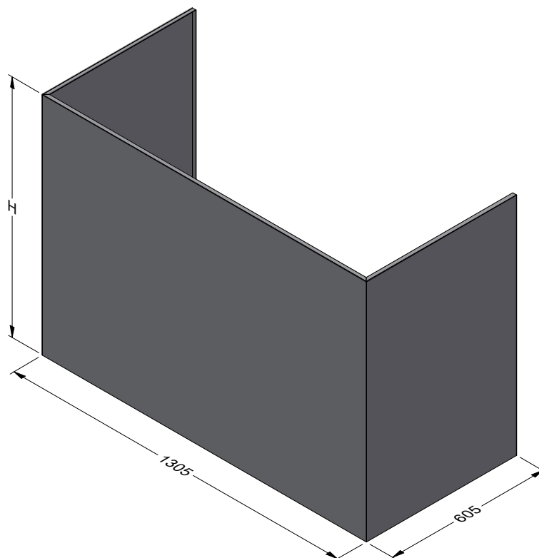
BCM 1500L-3 SHROUD
